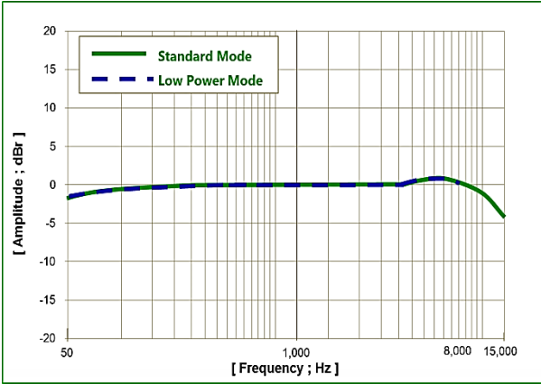
Figure 1. Typical Frequency Response, Normalized to 1kHz
